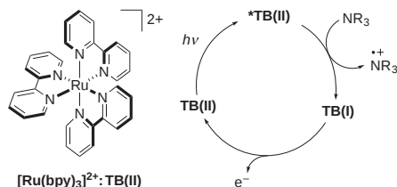
Scheme 1. Photosensitization process of TB(II).
