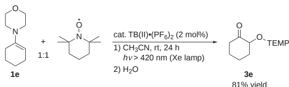
Scheme 3. Oxyamination of enamine derived from ketone.
