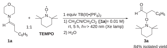
Scheme 2. Reaction of enamine with TEMPO in the presence of ^*\text{TB(II)} .
